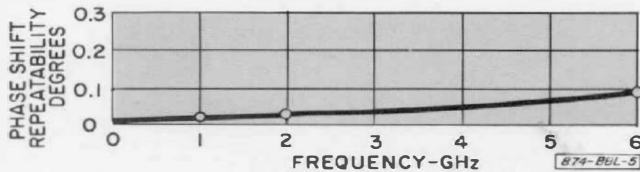
Figure 3. Phase-shift repeatability under same conditions.
