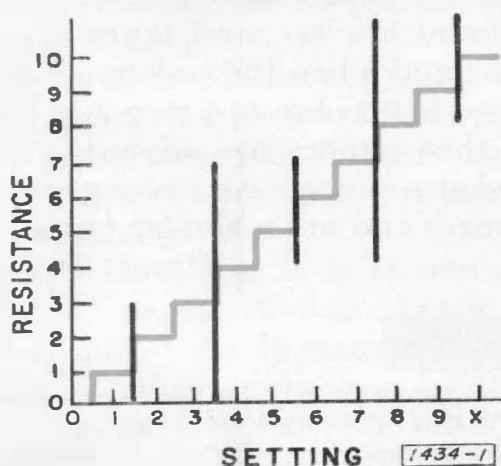
Figure 2. Limits of possible resistance jump during switching for a 1-2-4-4 combination. The system of Figure 3 avoids these jumps.
