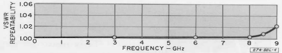
Figure 2. Repeatability, as a function of frequency, of the VSWR when the connection is repeatedly made and broken, for direct and 180° relative orientation of the connectors.
