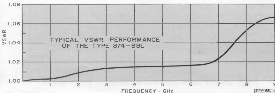
Figure 1. Plot of VSWR vs frequency for a typical mated pair of Type 874-BBL Coaxial Connectors.
