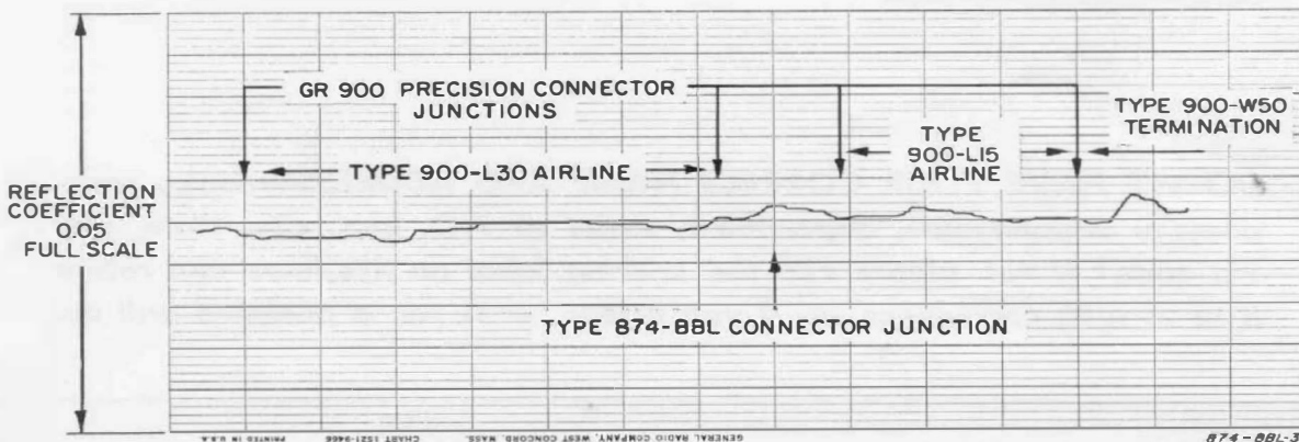
Figure 4. Time-domain reflectometer record for a pair of Type 874-BBL Coaxial Connectors inserted between two air-line sections equipped with GR900 Precision Coaxial Connectors.
