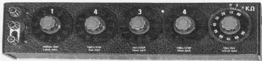
Figure 1. (right) Type 1434-QC Decade Resistor includes a continuously variable 100-ohm element (extreme right-hand dial). (below) The 7-dial Type 1434-G Decade Resistor can be used on the bench or in a rack. Photograph shows box with rack-mount hardware attached.
