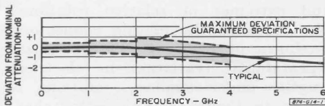
Figure 1. Attenuation vs frequency.
