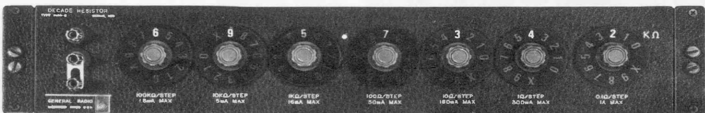
Figure 1. (right) Type 1434-QC Decade Resistor includes a continuously variable 100-ohm element (extreme right-hand dial). (below) The 7-dial Type 1434-G Decade Resistor can be used on the bench or in a rack. Photograph shows box with rack-mount hardware attached.
