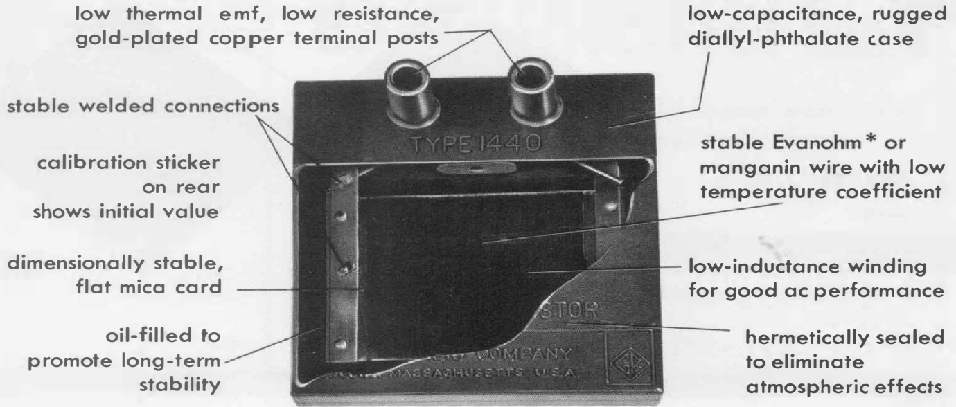
Figure 1. Cutaway view of the standard resistor, showing construction.
