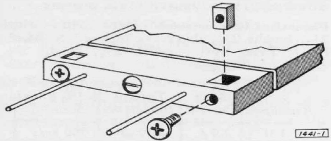
Figure 2. Type 1441 Standard Resistor can be mounted either vertically or horizontally. Hardware is furnished.
